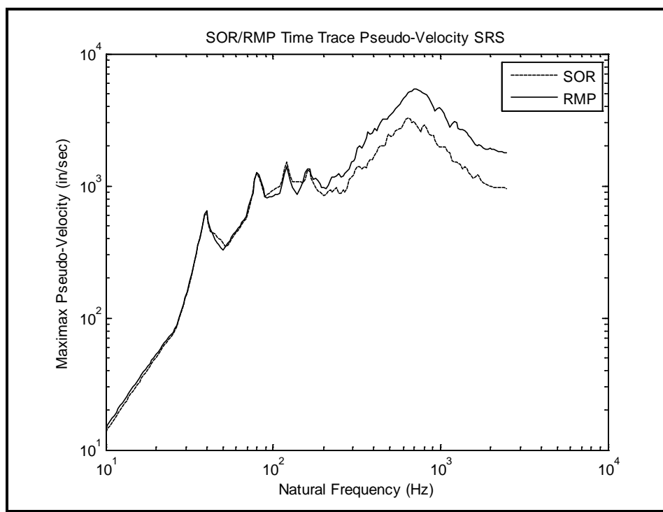
Figure 519.7C-10b. Pseudo-velocity shock response spectra for time trace.
