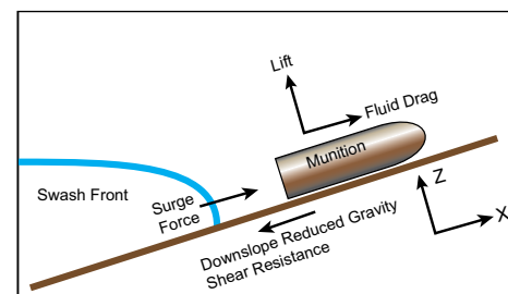
Schematic of the forces acting on a munition on a beach face.
